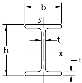
PulTex I-Sections
